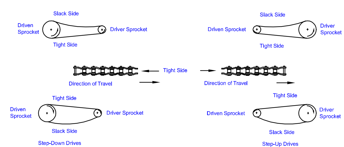
Direction of Drive Chain Travel as a Function of Wear
