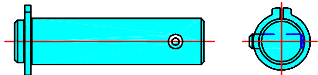
SNUB PIN WITH ANTI ROTATION FEATURE
