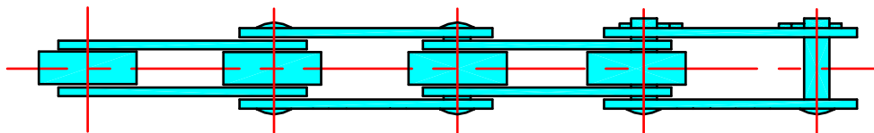
SOLID PINS
